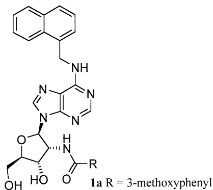
Figure 1. Lead structure 1a .
