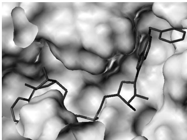
Picture 1. N^6 -benzyl NAD^+ -derivative inside L. mexicana GAPDH.
